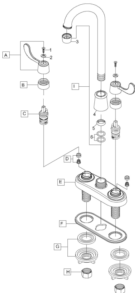
Complete Faucet #77791
